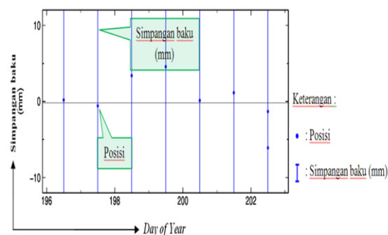
Gambar 6. Hasil plot time series komponen East
