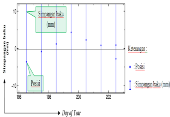
Gambar 5. Hasil plot time series komponen North
