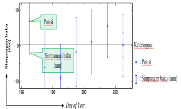
Gambar 7. Hasil plot time series komponen Up
