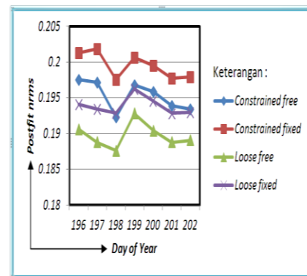
Gambar 3. Nilai postfit nrms
