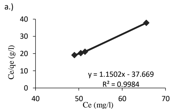
Gambar 6. (a)Isoterm Langmuir (b)Isoterm Freundlich adsorpsi logam besi menggunakan adsorben manganese zeolit 1,5 gram
