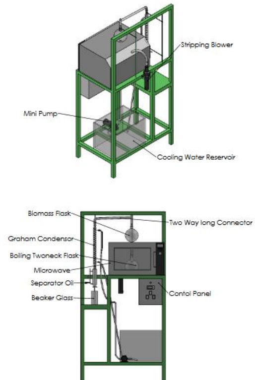
Gambar 1. Alat Microwave Hydrodistillation
