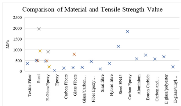
Figure 1. Comparison of Materials and Tensile Strength Value
