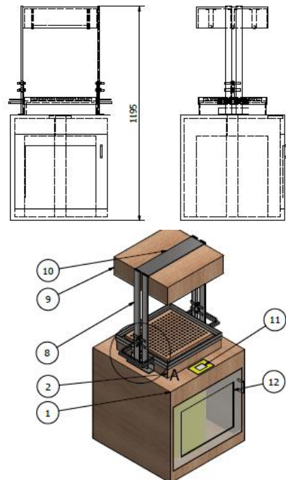
Gambar 2. Desain Alat Vacuum Forming
